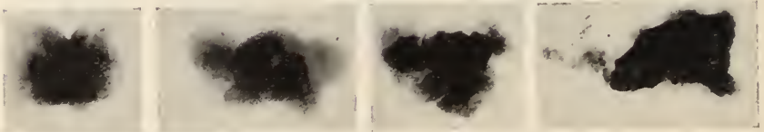
Strain TU
